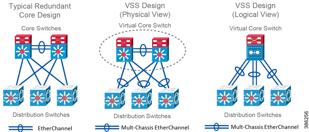
Figure 5 Core Switches—Traditional versus VSS Design
