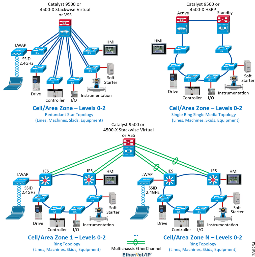
Figure 3 Catalyst 9500 or Catalyst 4500-X Aggregation/Distribution Switch
