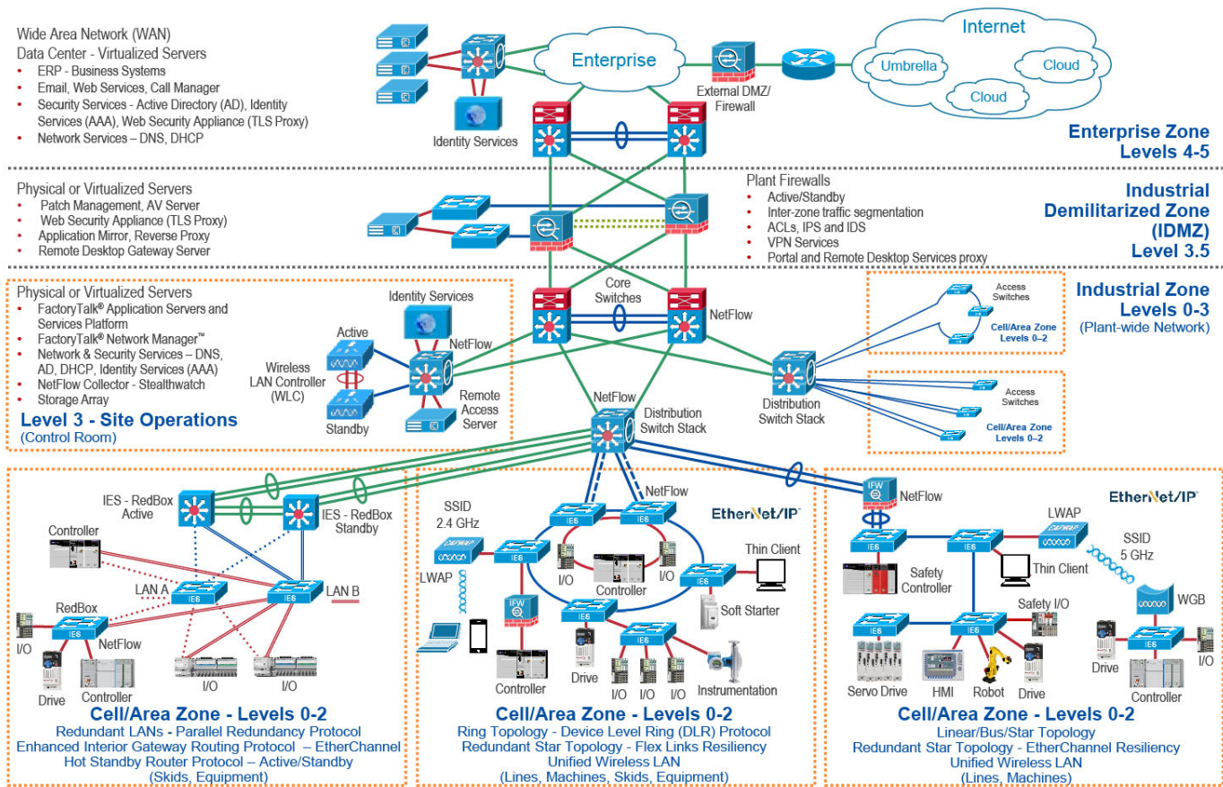
Figure 1 CPwE Architectures
