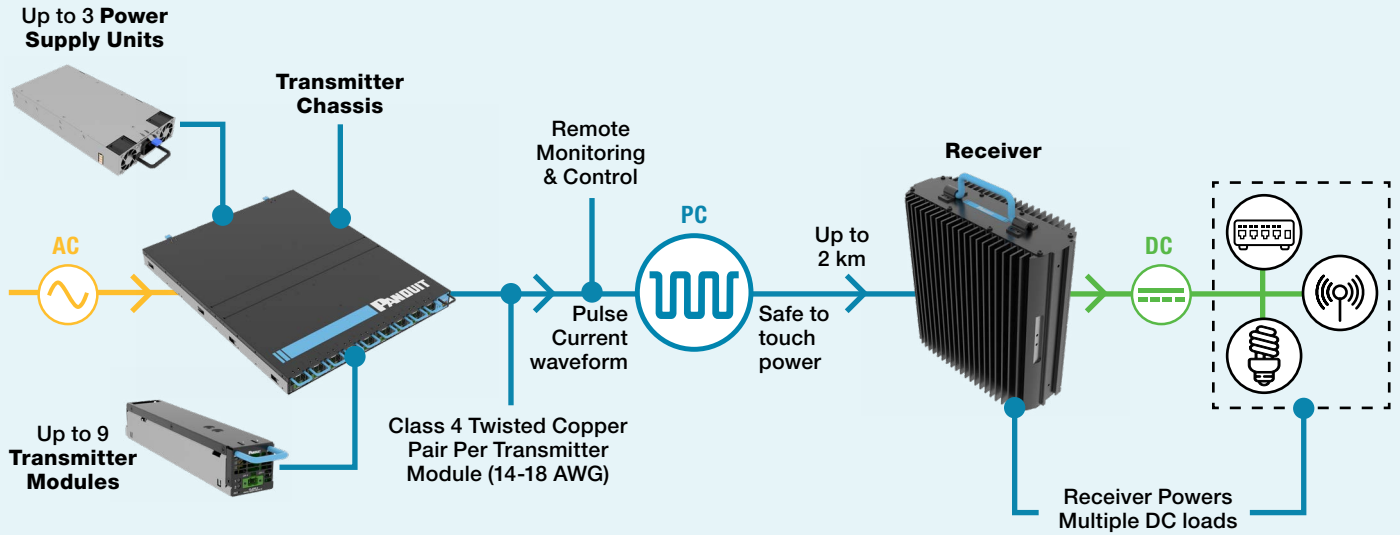
Figure 2: Overview of the Panduit FMPS, showing the Transmitter Chassis which typically resides in the headend, delivering power in a Pulse Current waveform, through multi-conductor cable, and sending it to the Panduit FMPS Receiver which is typically distributed throughout the building near devices that require power.
