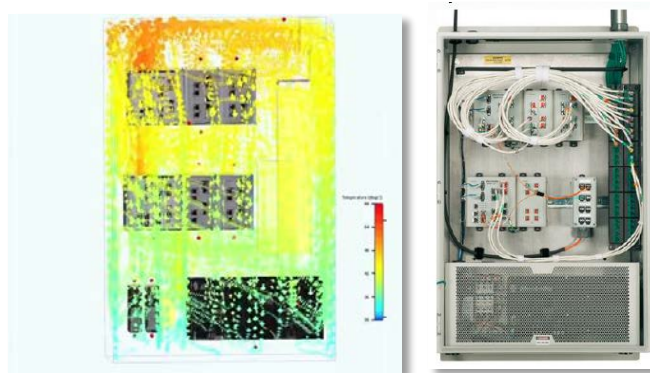
Figure 4: Example of Computational Fluid Dynamics (CFD) used to verify all temperatures below maximum operating temperature, (none in red) over time and under simulated operating conditions.
