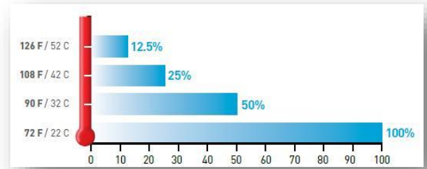
Figure 1: Electronics life expectancy percentage (Source: Digital Equipment Corporation).
