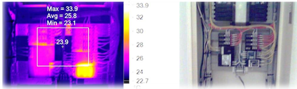
Figure 5: Example of infrared thermal imaging used to evaluate existing panel designs in operation.
